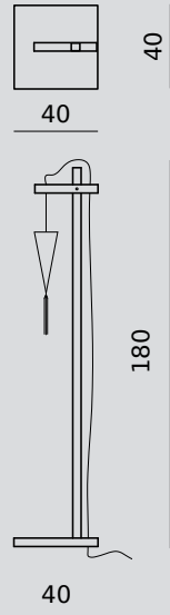
PIANTANA FLOOR SUPPORT SU.FL
